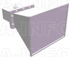
LB-650-10-C-SFSPO Standard Gain Horn Antenna 1.12-1.7GHz 10dB Gain SMA Female
